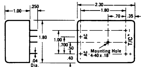
Case Size ES-10
